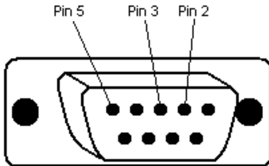
RS232 connector (female)
